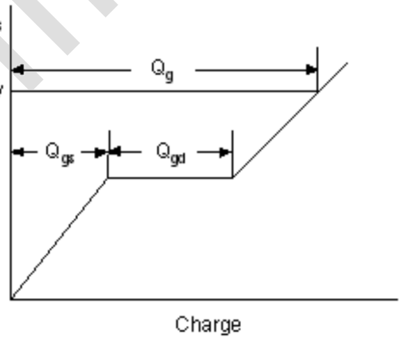
Figure 15. Gate Charge Test Circuit & Waveform
